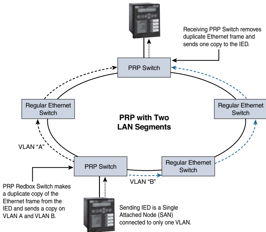
Figure 11-8 PRP Deployment Example
