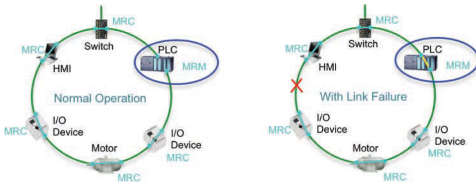
Figure 9-10 PROFINET MRP Operation
