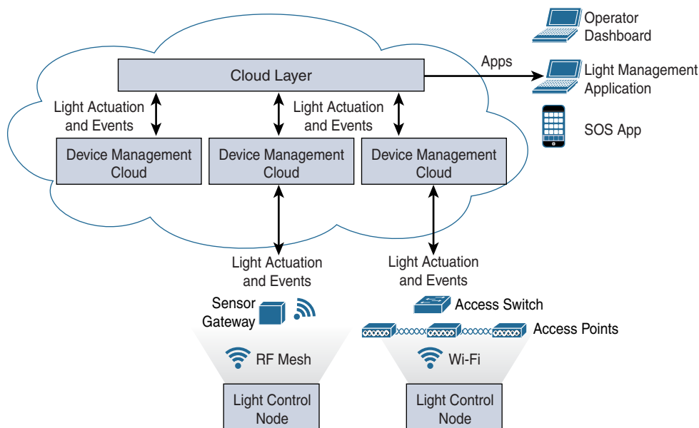
Figure 12-7 Connected Lighting Architecture
