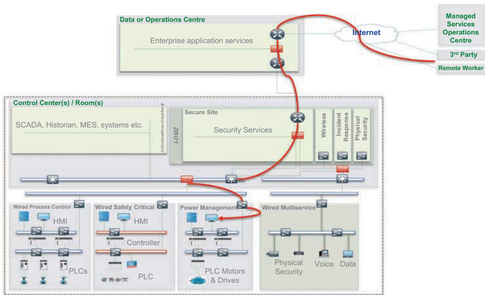
Figure 10-17 Remote Access Session Flow into the PCN
