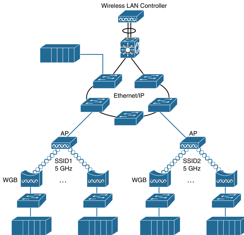
Figure 9-8 A Factory Wireless LAN Architecture
