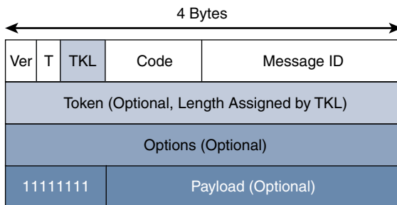
Figure 6-7 CoAP Message Format
