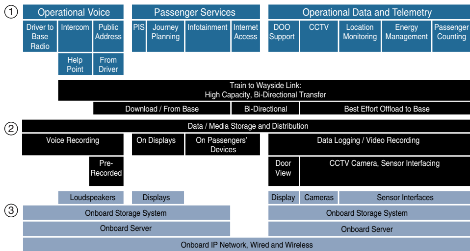
Figure 13-11 Train IoT Technology Components
