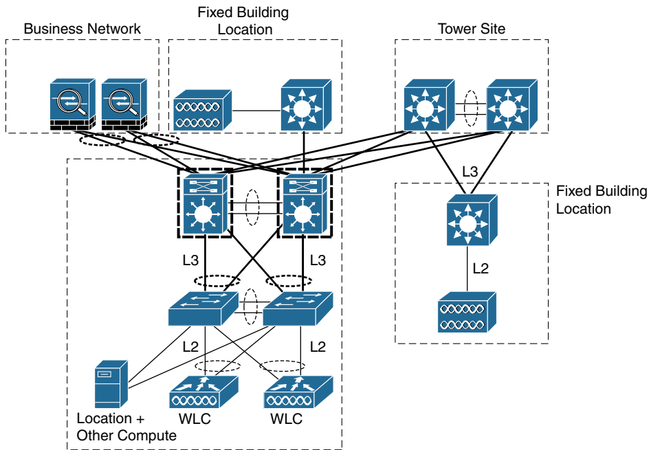
Figure 14-23 Common Core Network Deployment for Mining
