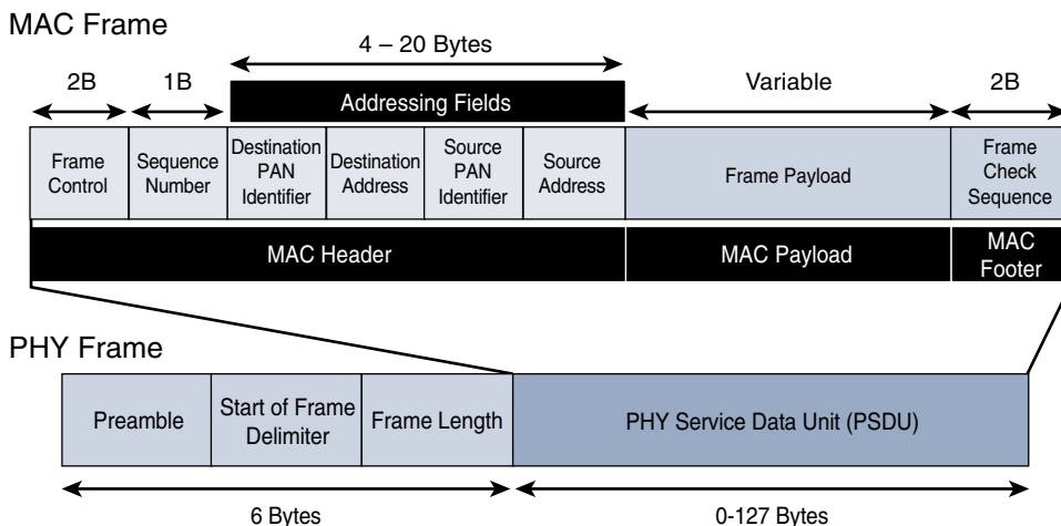
Figure 4-6 IEEE 802.15.4 MAC Format
