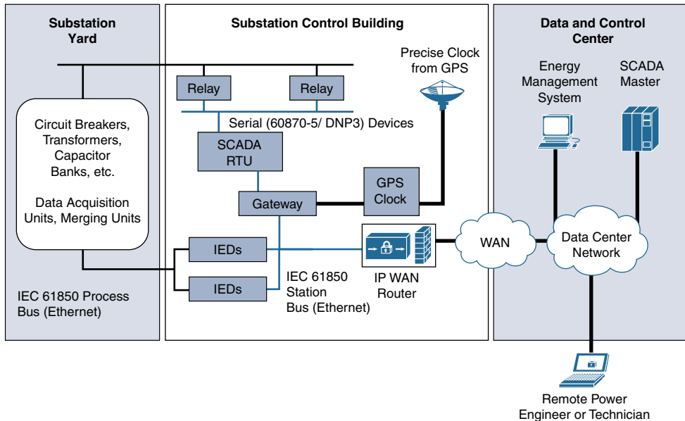
Figure 11-7 The IEC 61850-Based Substation Architecture
