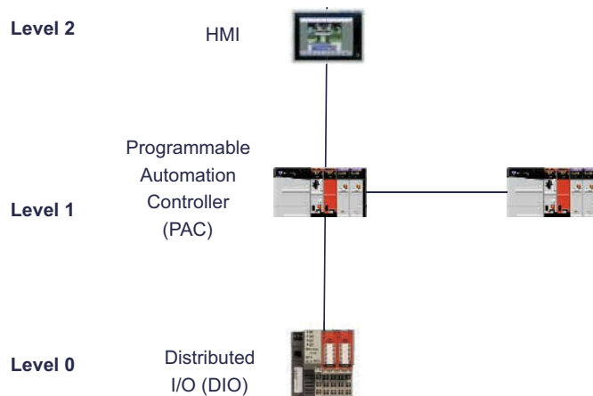
Figure 9-4 IACS Controller Traffic Flow
