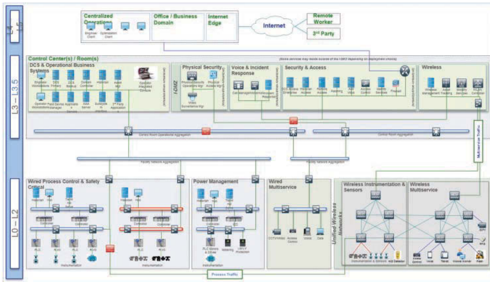
Figure 10-12 An Oil and Gas Reference Architecture
