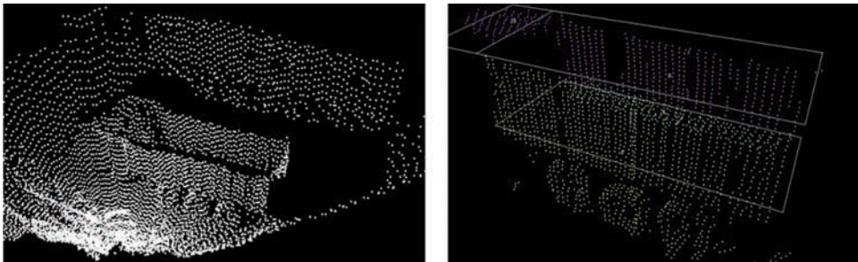
Figure 14-18 Sensors for Truck Loading
