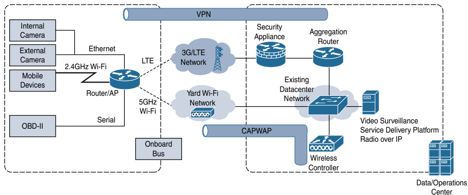
Figure 15-18 Connected School Bus Network Architecture
