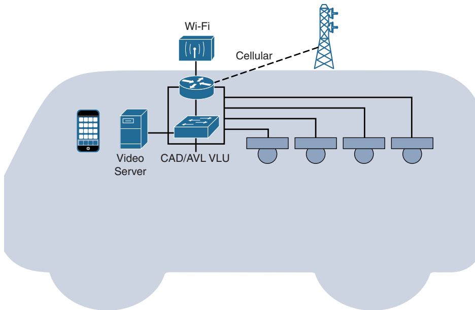
Figure 13-10 Mass Transit: Bus Onboard System Architecture
