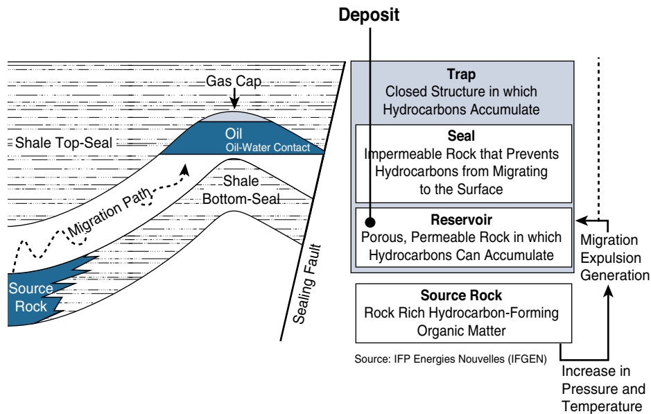
Figure 10-2 From Organic Matter to Oil and Gas
