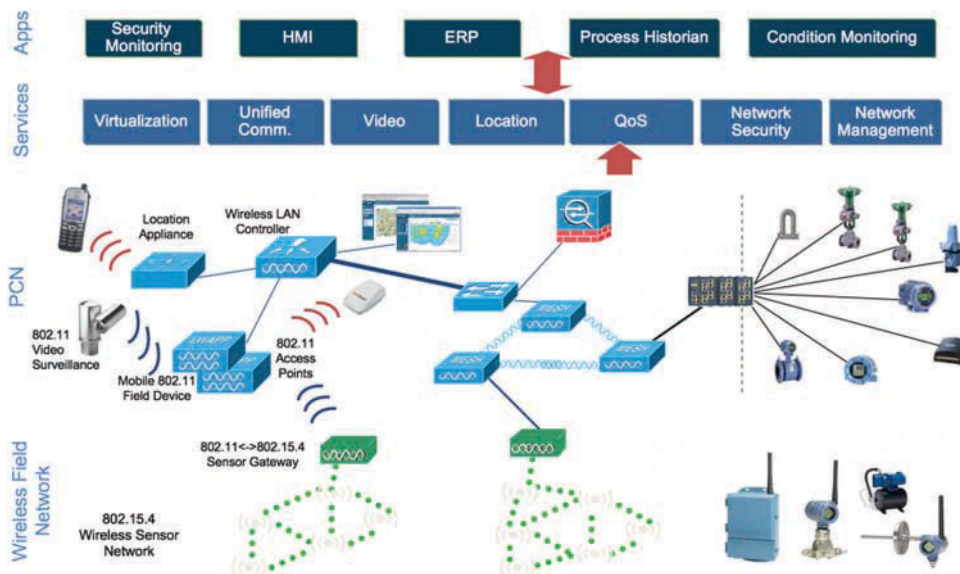
Figure 10-13 WFN Mesh Architecture in an 802.11 Wireless Mesh
