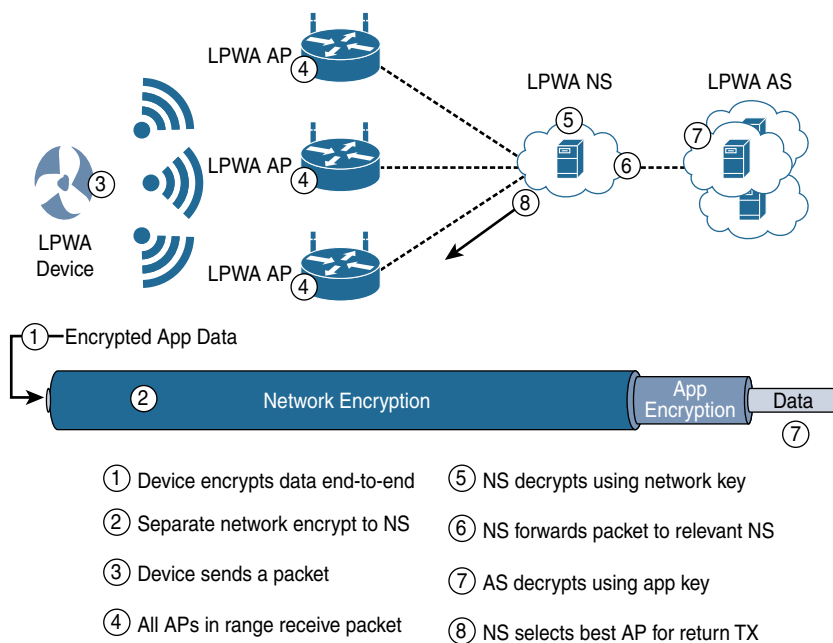
Figure 4-18 LoRaWAN Security
