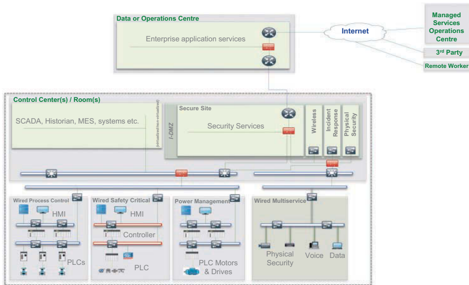
Figure 10-16 Security Operations Reference Architecture
