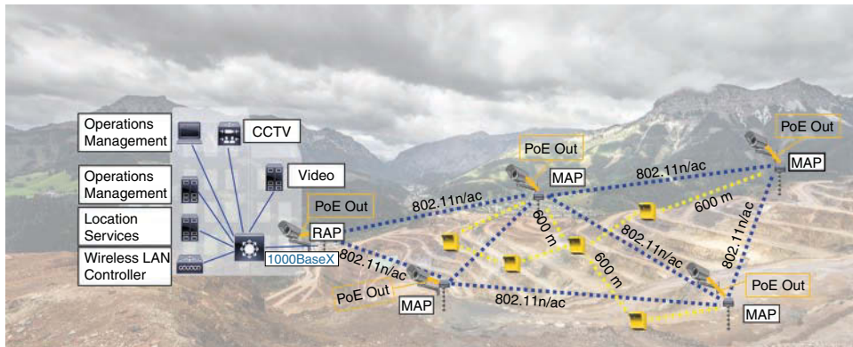
Figure 14-21 Simple Mine Topology, with No Connections to External Networks
