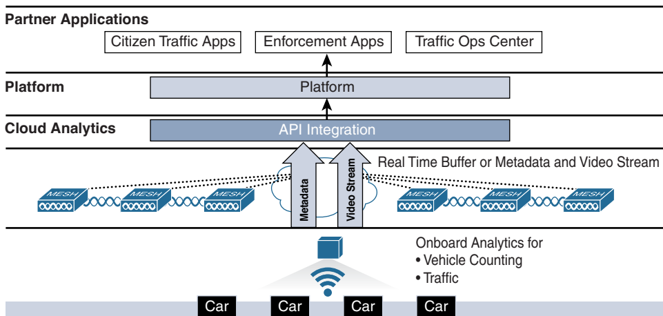
Figure 12-9 Smart City Traffic Architecture
