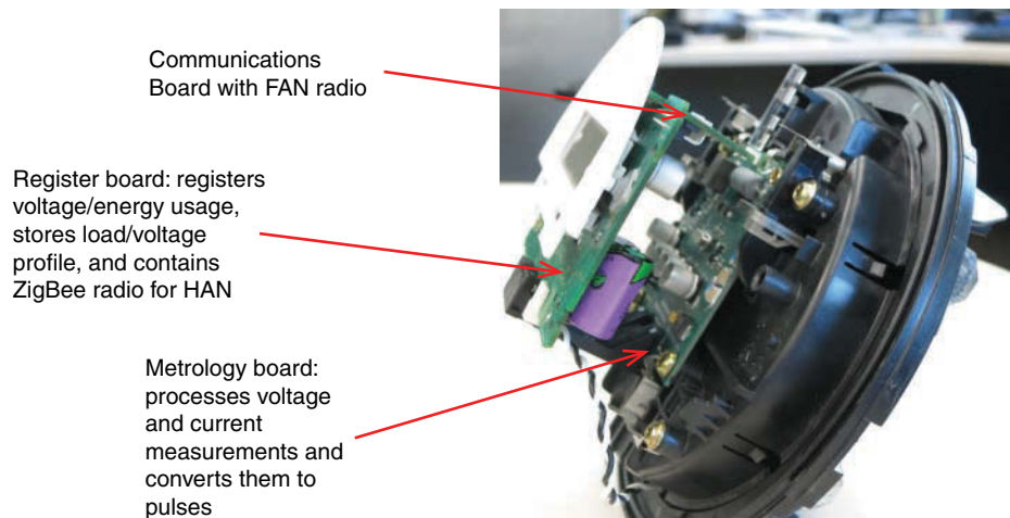
Figure 11-15 The Anatomy of a Smart Meter
