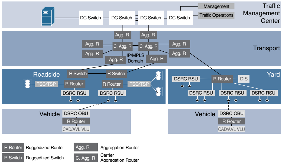
Figure 13-7 Connected Roadways IoT Network Architecture
