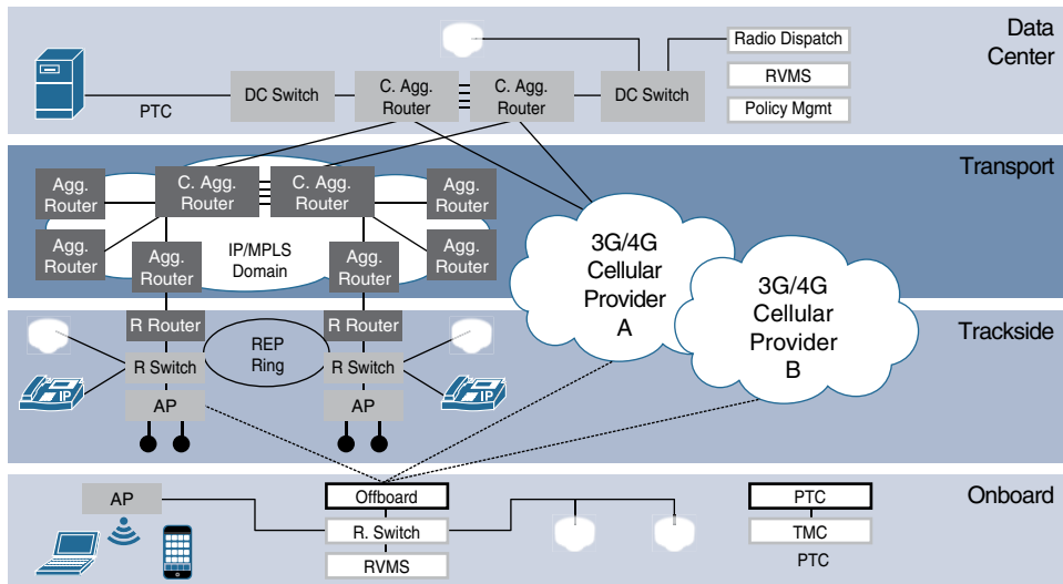
Figure 13-12 Connected Rail IoT Architecture
