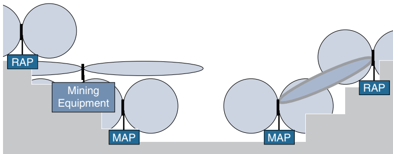
Figure 14-19 Antennas and Coverage Limits in Three-Dimensional Spaces
