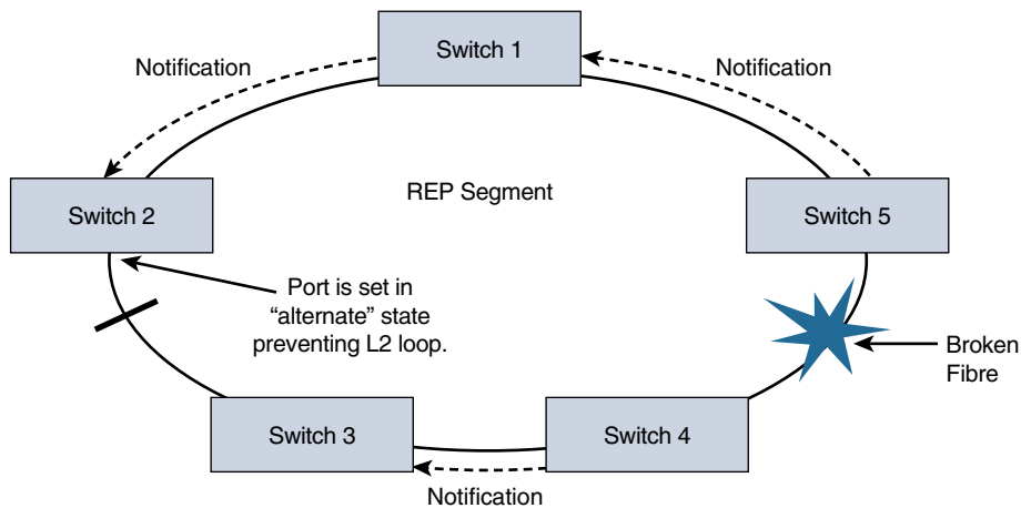
Figure 9-6 REP Notification When a Topology Change Occurs
