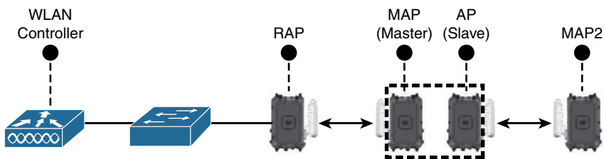
Figure 14-16 MAP Daisy-Chaining Topology
