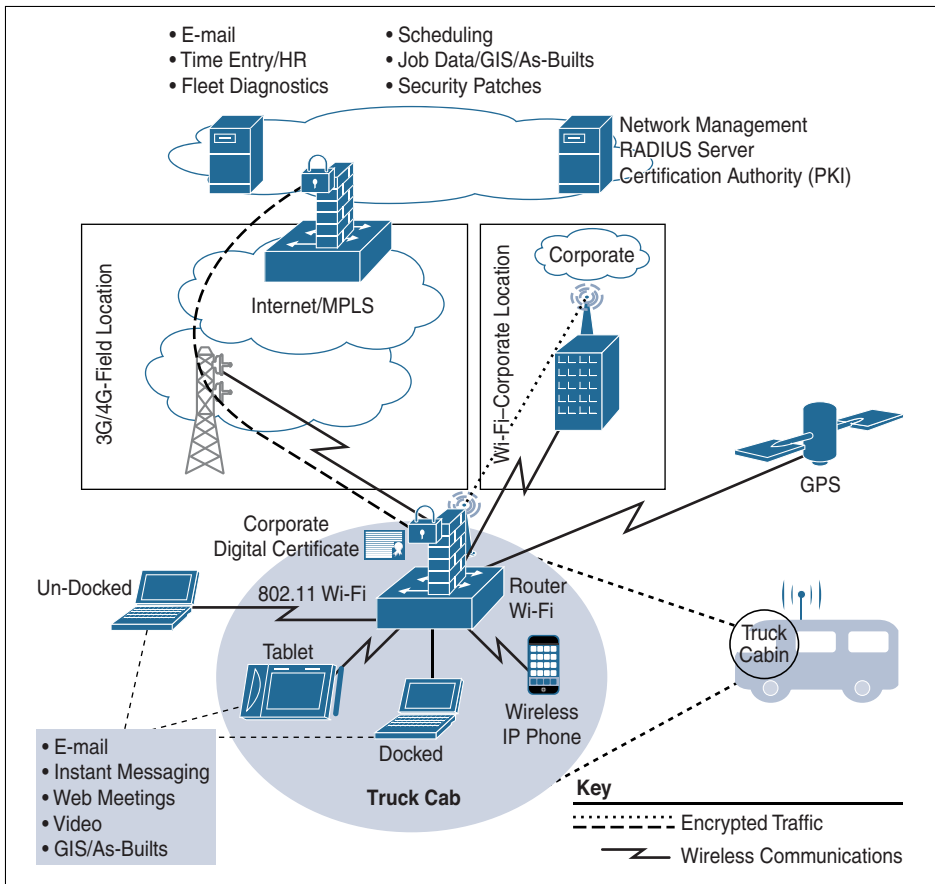
Figure 13-8 Fleet Management Architecture
