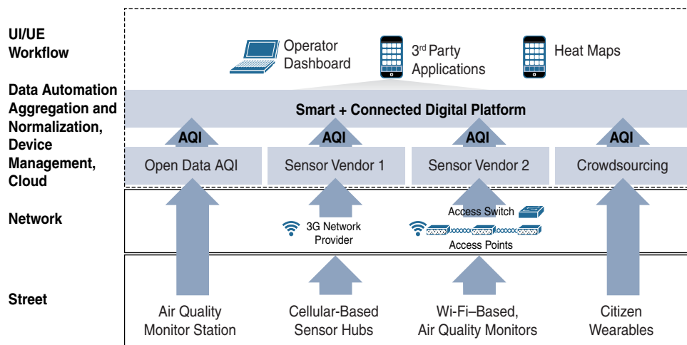
Figure 12-10 Connected Environment Architecture
