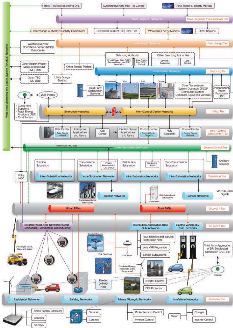
Figure 11-2 The GridBlocks Reference Architecture
