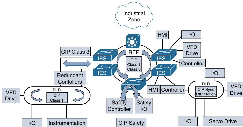
Figure 9-9 A Factory Network Based on EtherNet/IP
