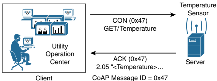
Figure 6-9 CoAP Reliable Transmission Example
