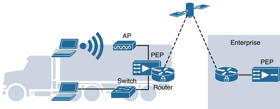
Figure 15-7 Wi-Fi and Satellite Communication Architecture
