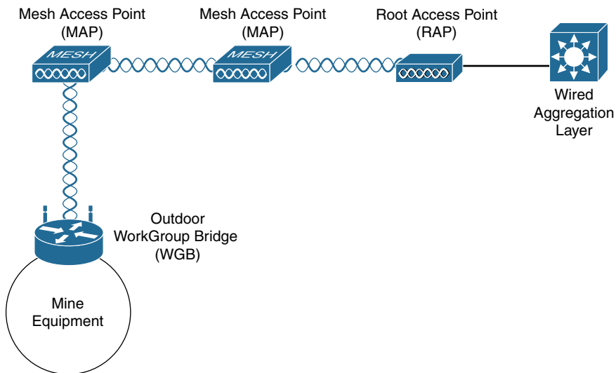
Figure 14-14 Wi-Fi Mesh Architecture for Mining
