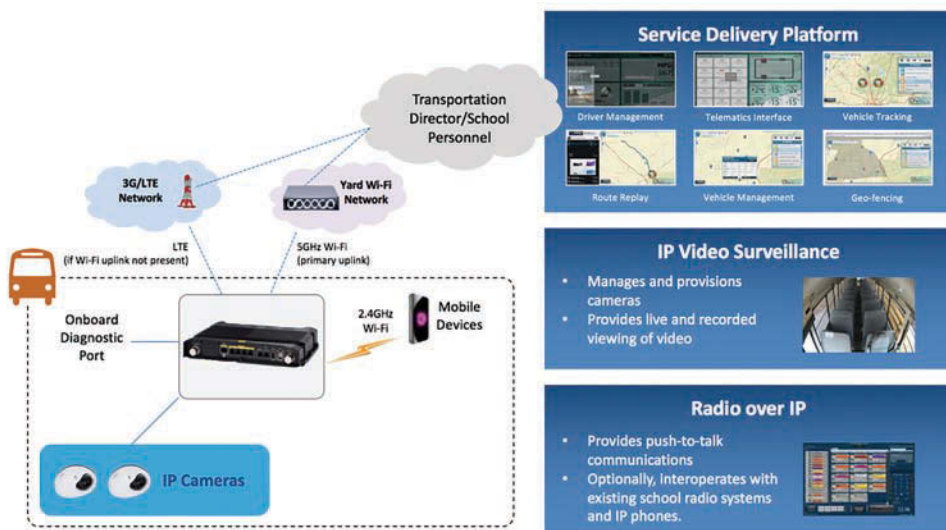
Figure 15-12 School Bus Safety Communication Architecture
