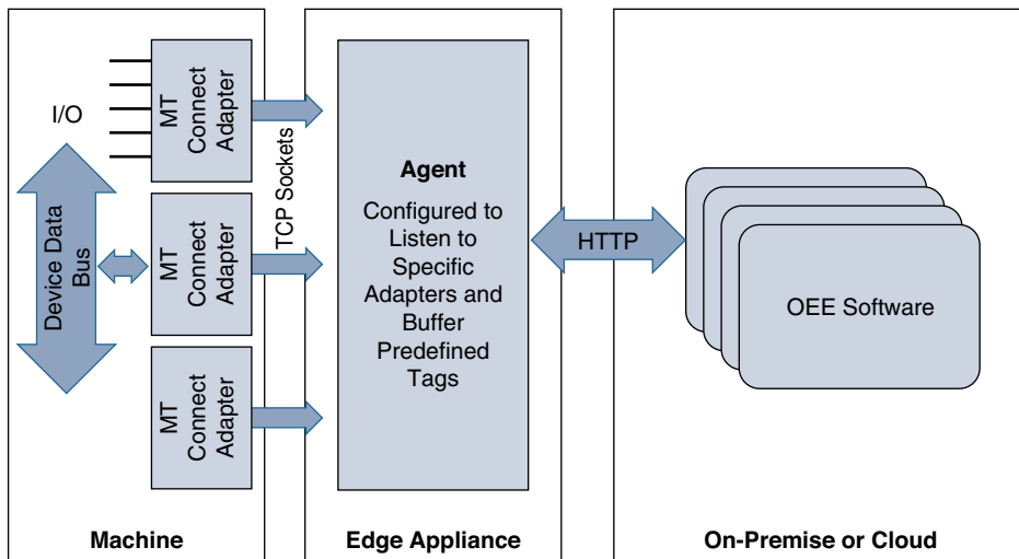
Figure 9-13 Connected Machine Model Based on MTConnect
