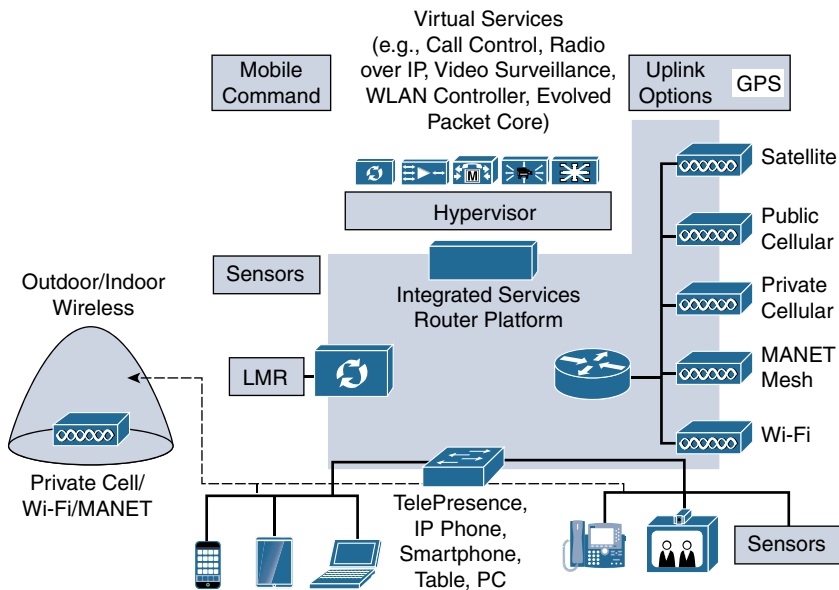
Figure 15-4 Mobile Command Center
