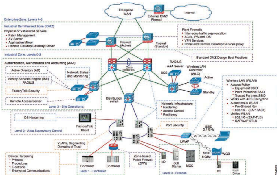
Figure 9-11 Industrial Network Security Framework
