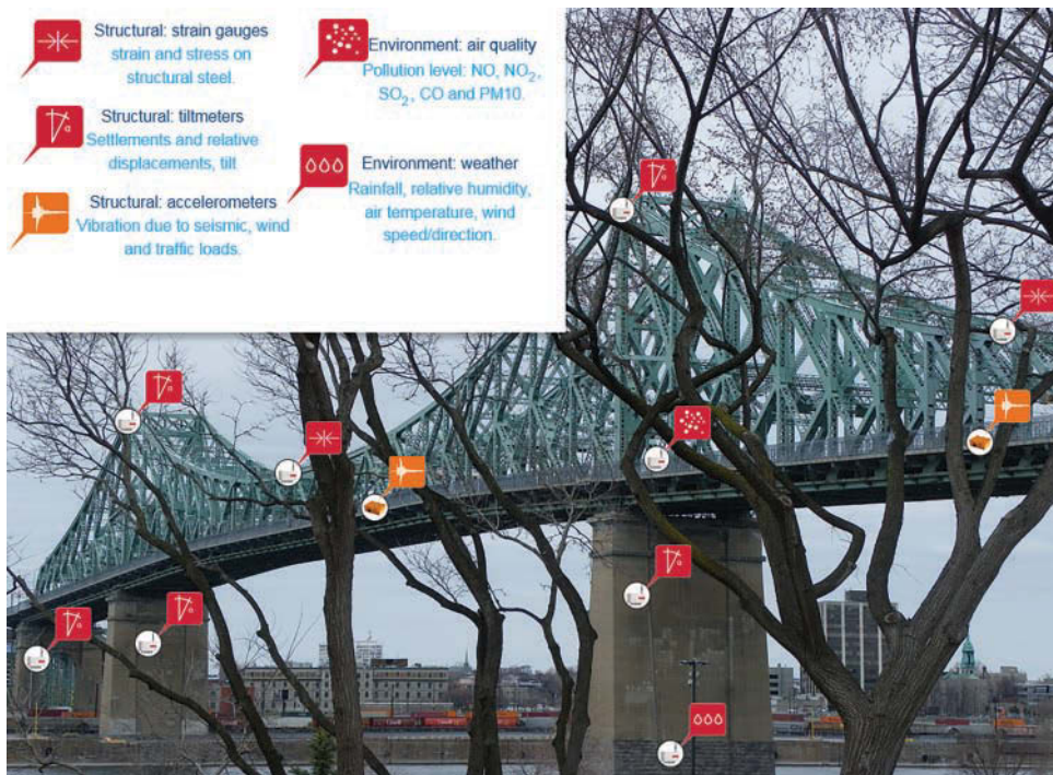
Figure 13-2 Smart Objects Monitoring a Bridge
