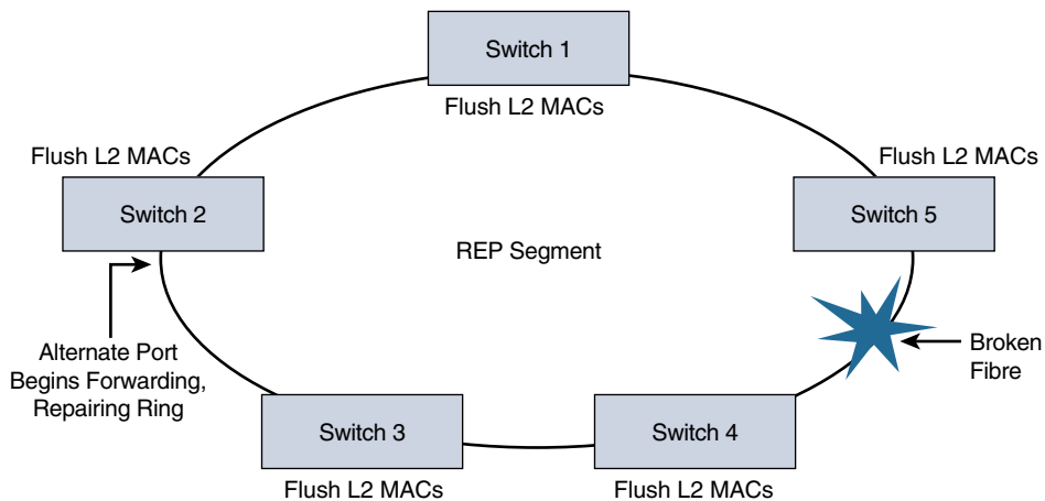
Figure 9-7 Reconvergence of the REP Ring Segment
