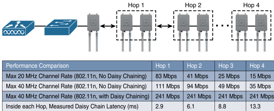
Figure 14-17 Daisy Chaining MAPs in a Wireless Mesh Deployment
