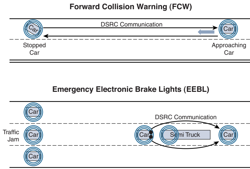
Figure 13-4 DSRC Emergency Brake Warnings
