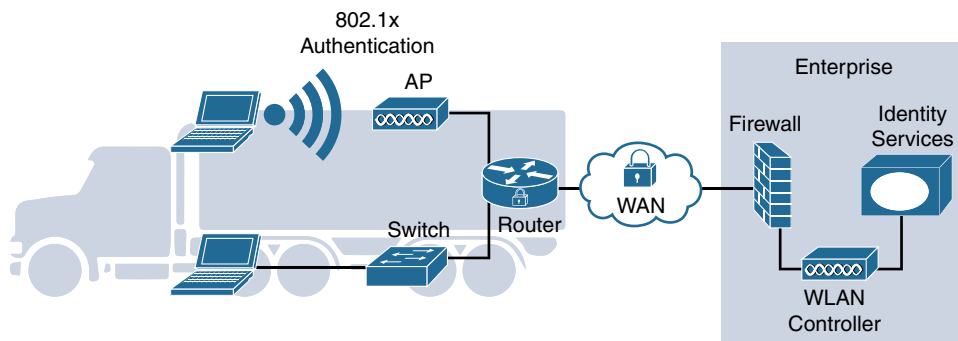
Figure 15-6 Wi-Fi Communication Architecture
