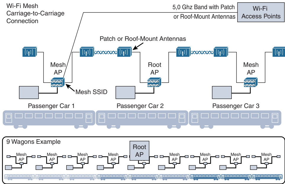
Figure 13-14 Carriage-to-Carriage Wi-Fi for Connected Trains
