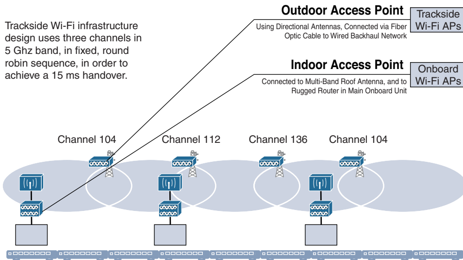
Figure 13-16 Connection to Trackside Wi-Fi Network
