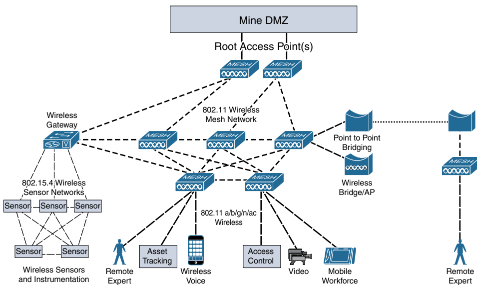
Figure 14-20 Network Topology of a Combined IEEE 802.11 and IEEE 802.15.4 Industrial Wireless Solution
