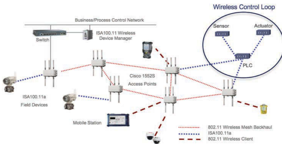
Figure 10-14 An Example of a Combined Wi-Fi with ISA100.11 Network
