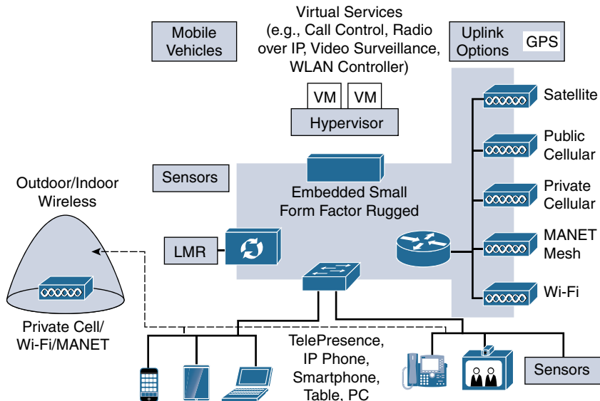
Figure 15-10 Land, Air, and Sea Mobile Vehicles
