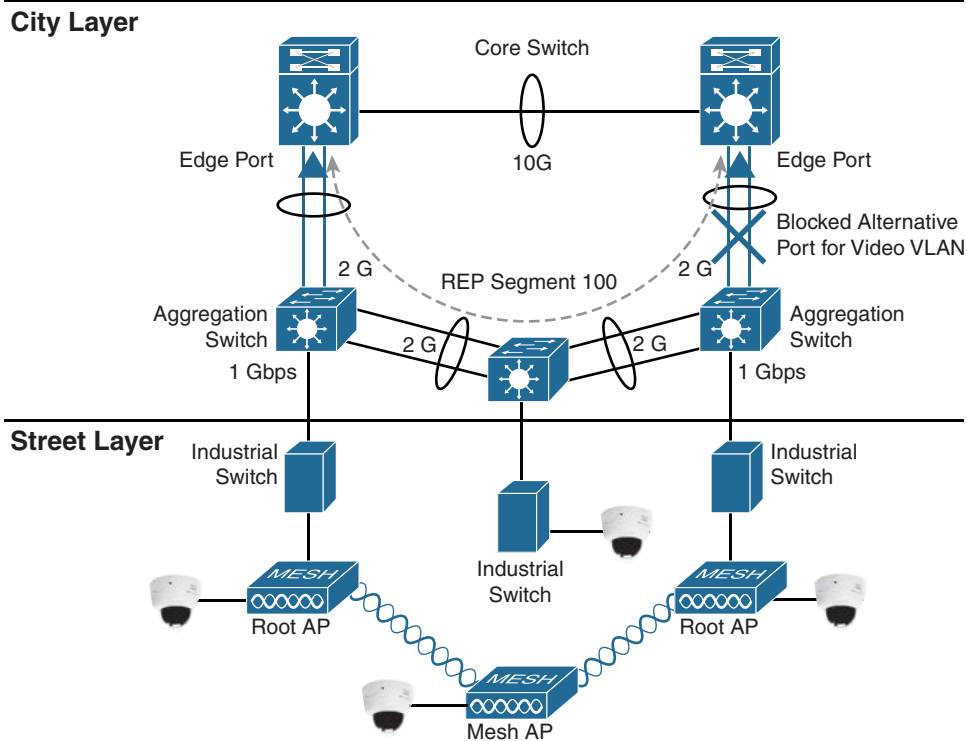
Figure 12-3 Street Layer Resiliency
