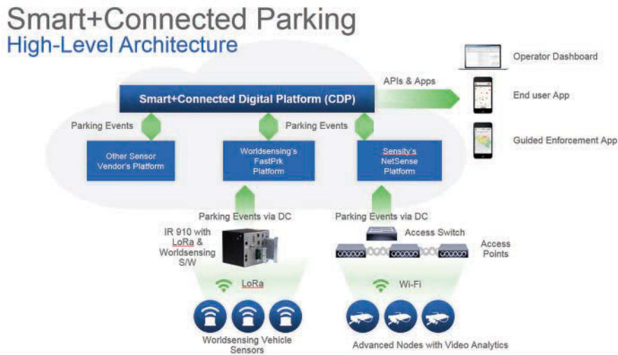
Figure 12-8 Connected Parking Architecture
