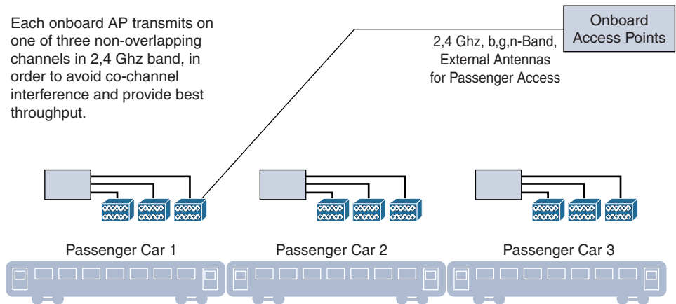
Figure 13-15 Onboard Wi-Fi
