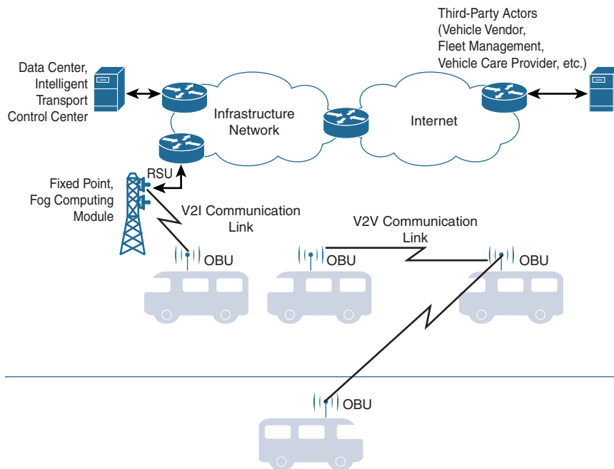
Figure 13-3 DSRC General Communication Architecture
