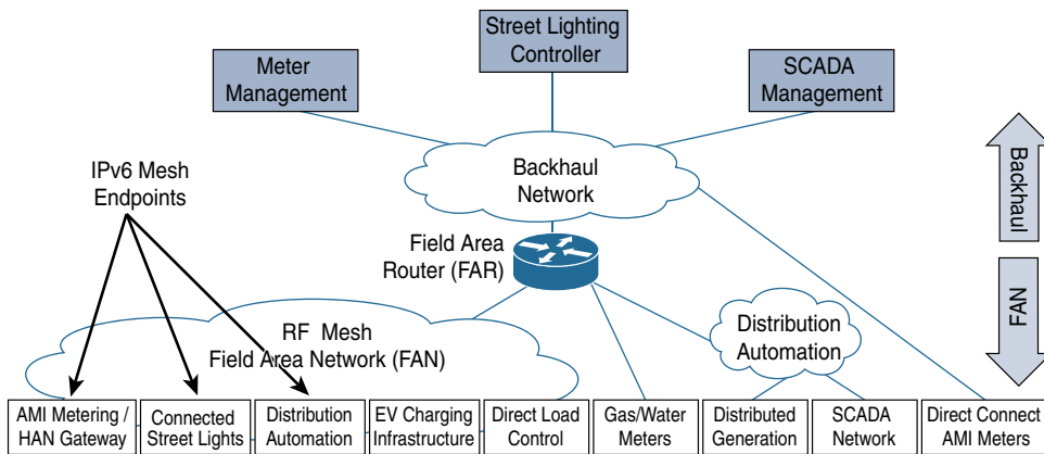
Figure 11-13 The FAN Multiservice Grid Network
