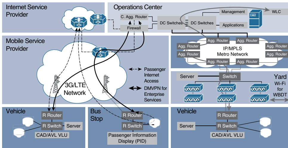
Figure 13-9 Connected Fleet Architecture
