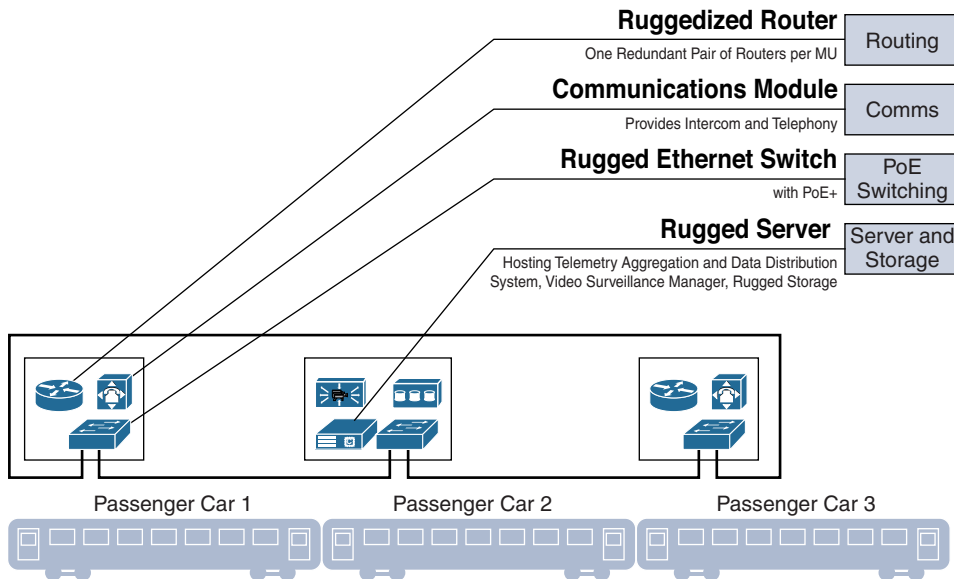
Figure 13-13 Semi-Distributed Onboard IoT Modular Architecture for Trains
