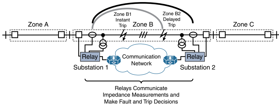
Figure 11-9 A Sample Distance Protection Scheme
