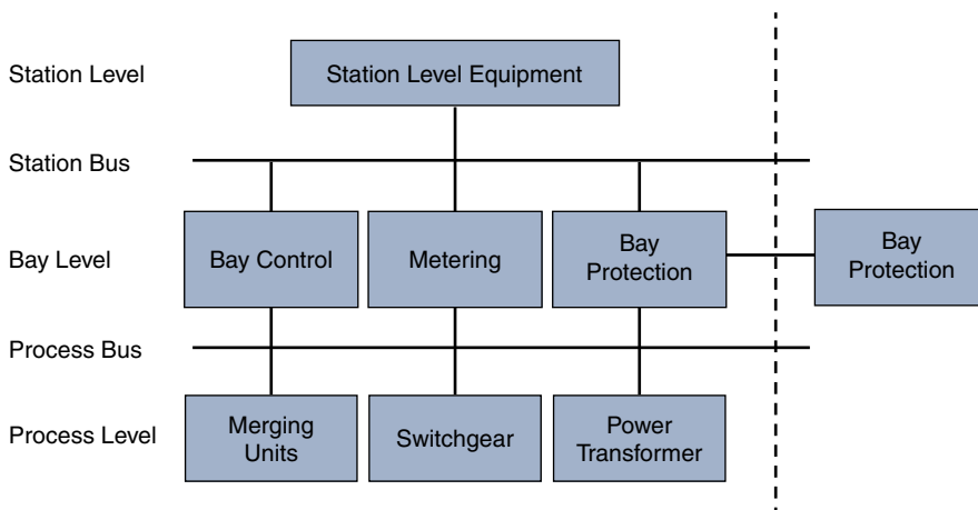
Figure 11-6 Substation Automation Hierarchy
